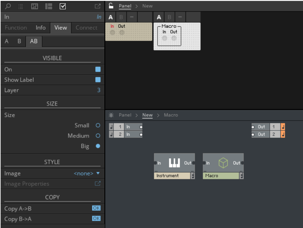
Ports of an Instrument and a Macro made visible on the panel
