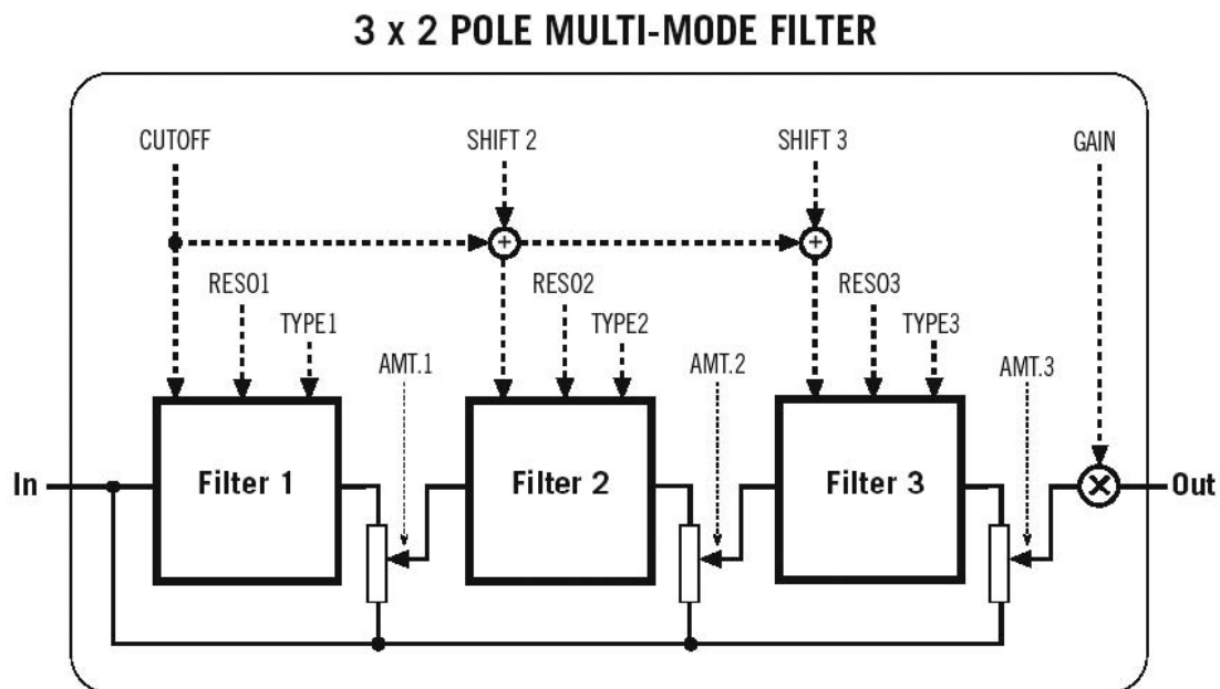
The basic internal signal flow structure of the 3x2 Pole Multi-Mode Filter
