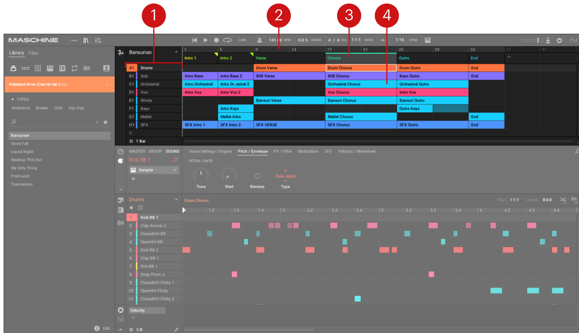
The Song view of a Maschine Project.
