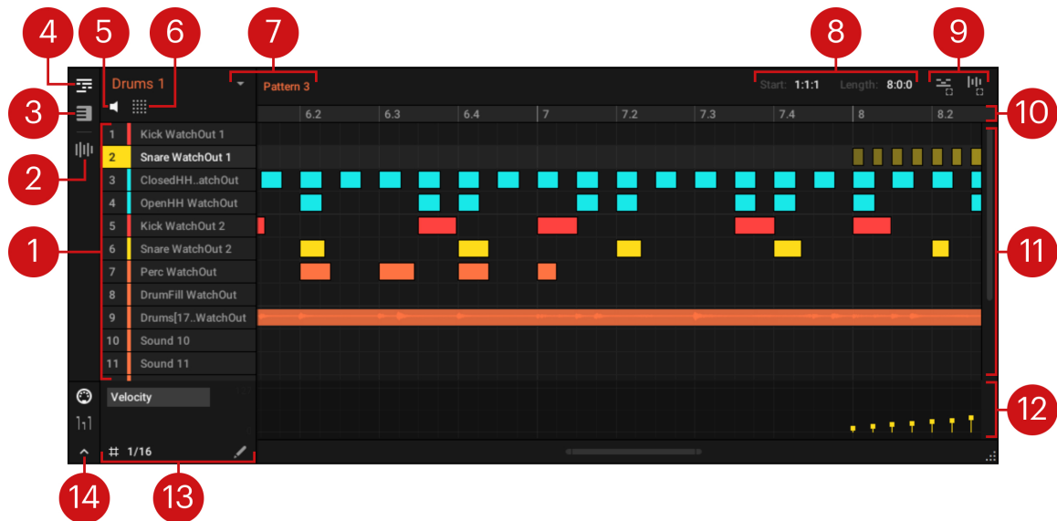
The Pattern Editor
