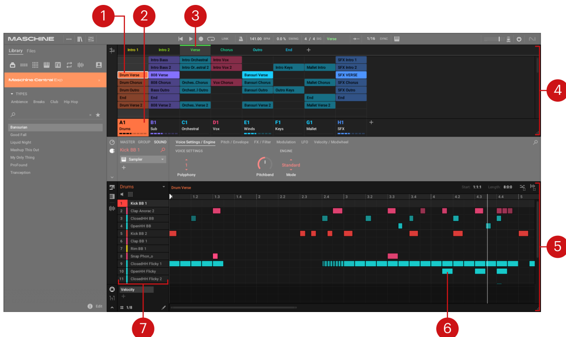
The Ideas view of a Maschine Project optimized for creating Patterns and building Scenes.
