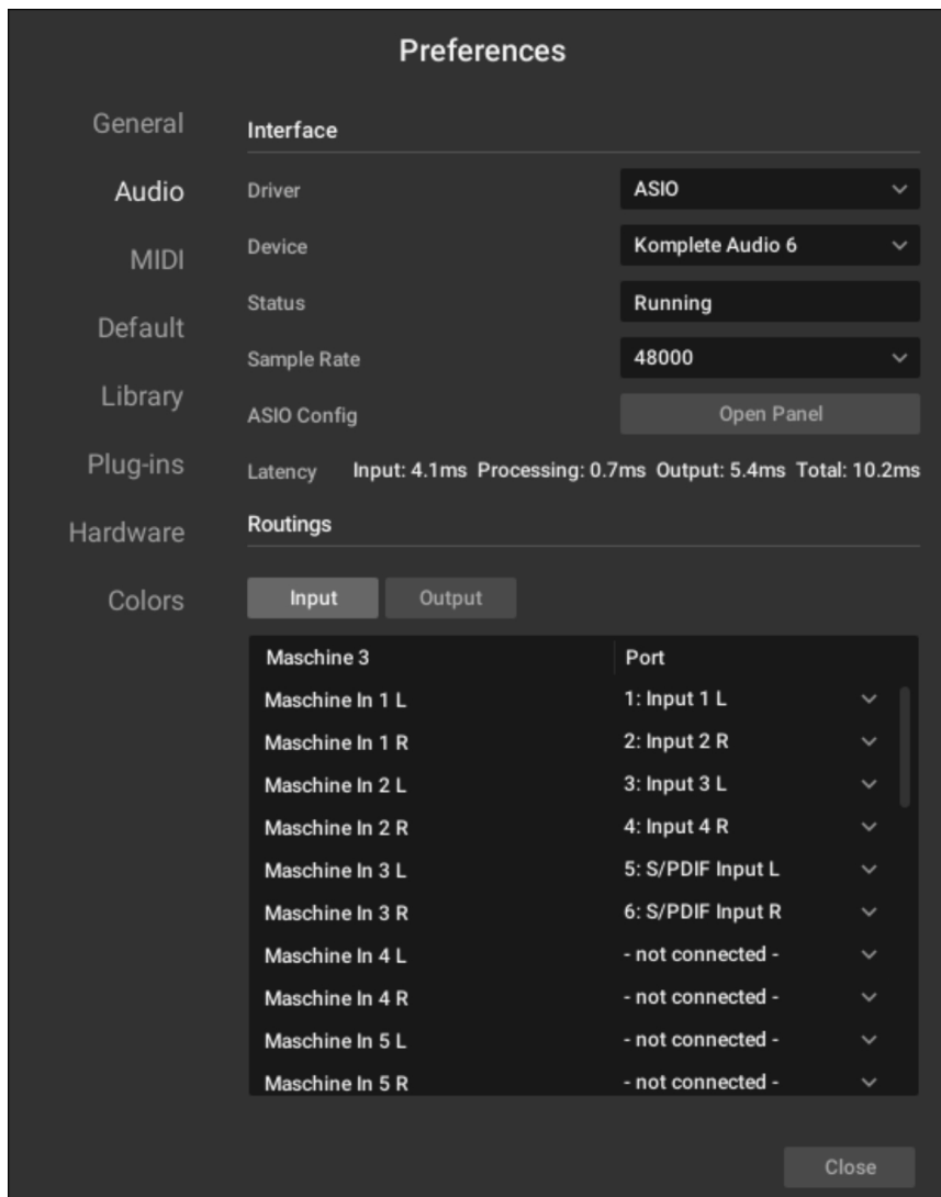
Preferences – Audio page.
