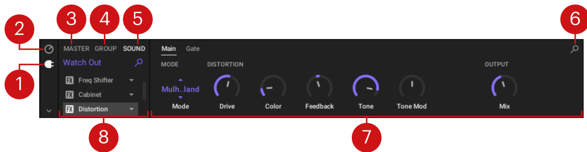
The Control area
