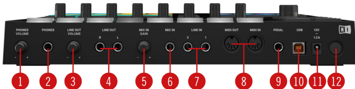
The rear panel of the Maschine controller.
