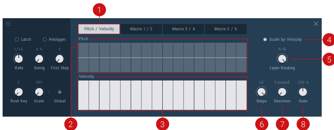
Sequencing Pitch in the Sequencer
